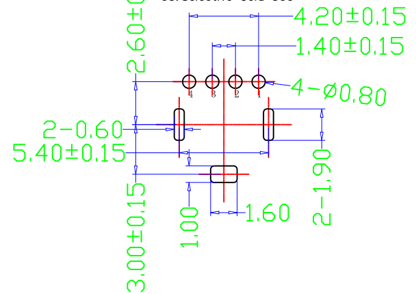
RECOMMENDED PCB LAYOUT GENERAL TOLERANCES: \pm 0.05
